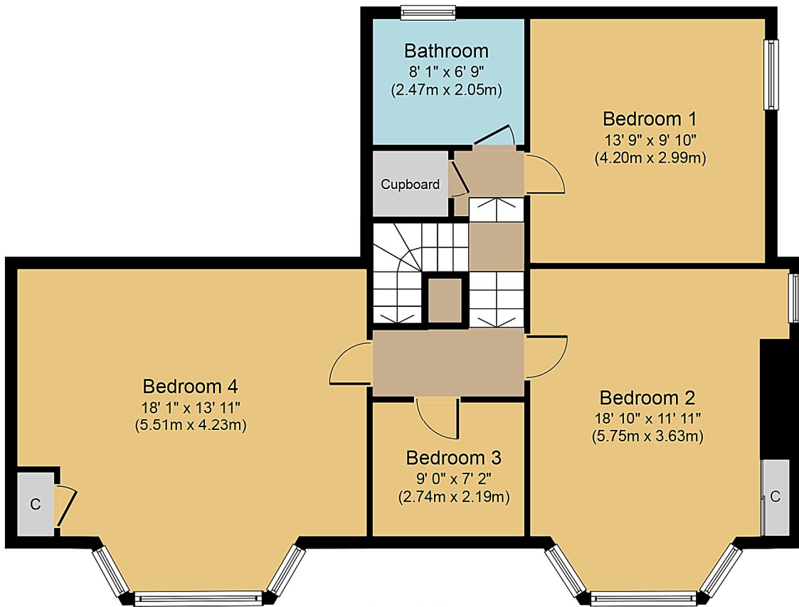
First Floor Approximate Floor Area 926 sq. ft. (86.0 sq. m.)
